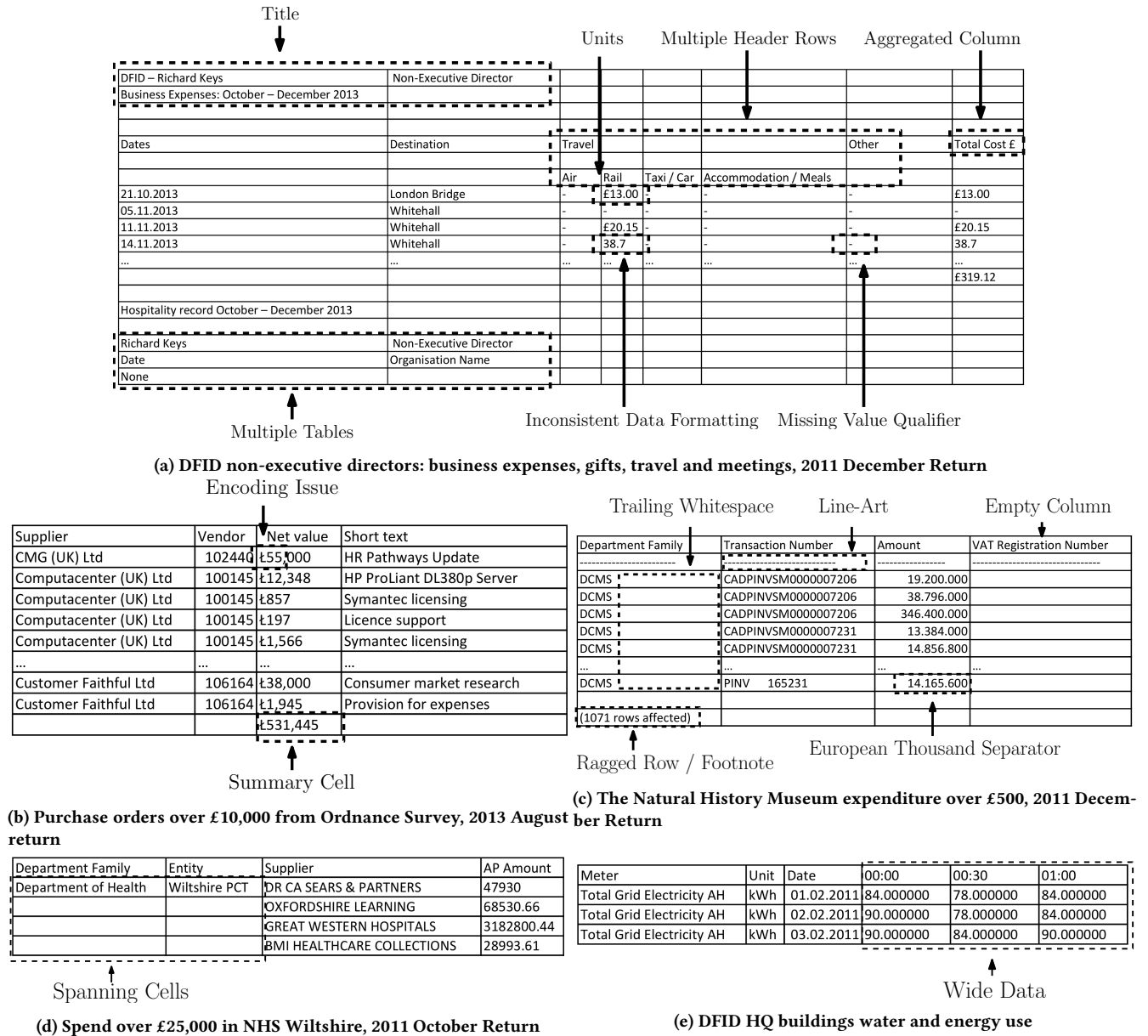
Figure 2: Tables from data.gov.uk illustrating a multitude of issues
