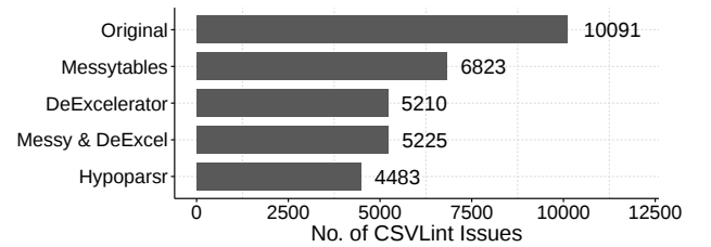
Figure 12: CSVLint issues after parsing and writing back to RFC4180-conform CSV.
