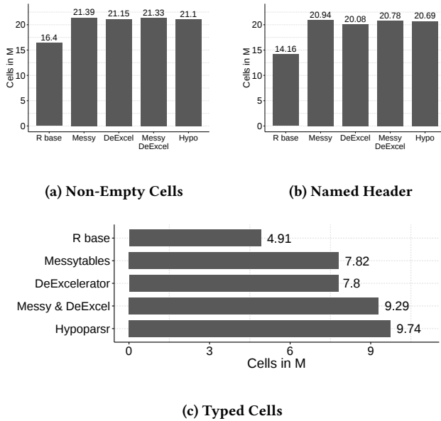
Figure 10: Amount of recovered data cells from data.gov.uk corpus with hypoparsr and compared solutions.
