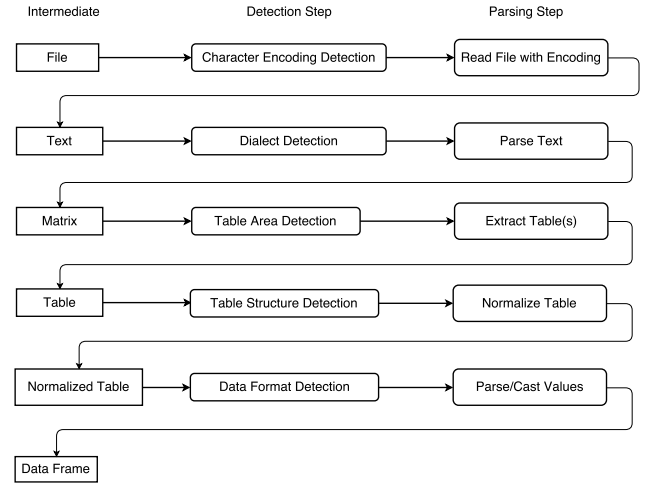
Figure 4: Parsing steps of hypoparsr . Table structure detection summarizes the detection of row and column functions.
