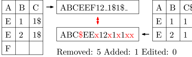
Figure 9: String-based table distance measure.
