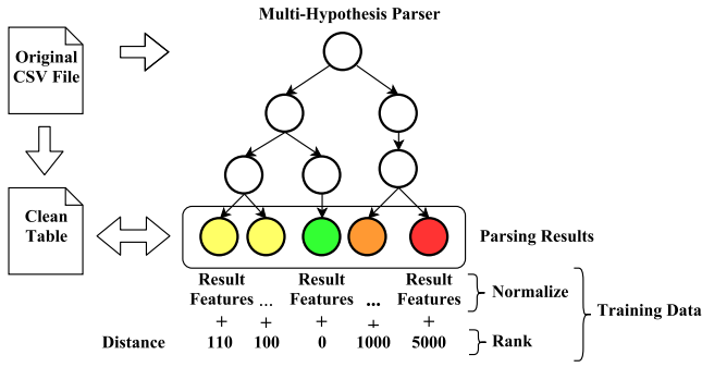
Figure 6: Schematic diagram of the training data generation process.
