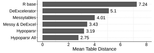
(b) Mean distance to cleaned tables.
