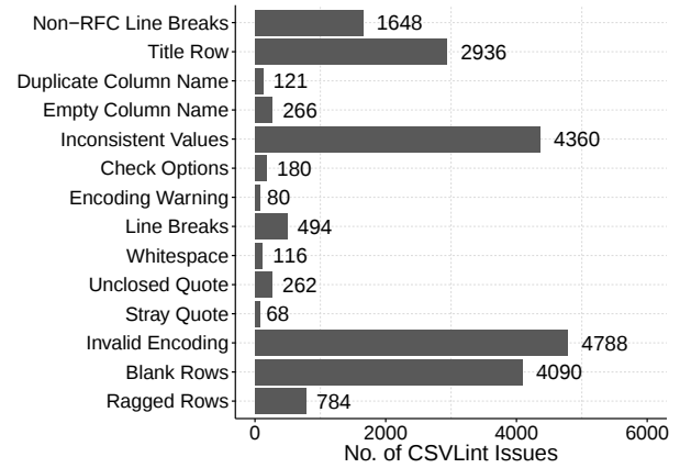
Figure 11: CSVLint issues in the data.gov.uk corpus.
